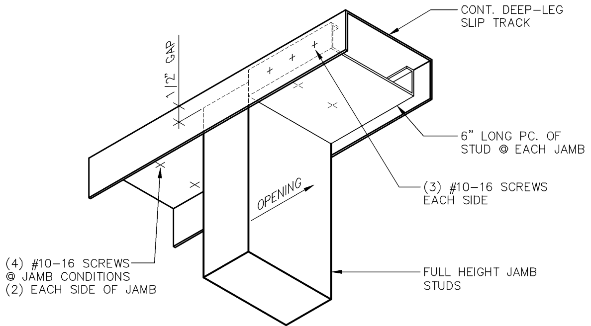
@ JAMB CONDITIONS
