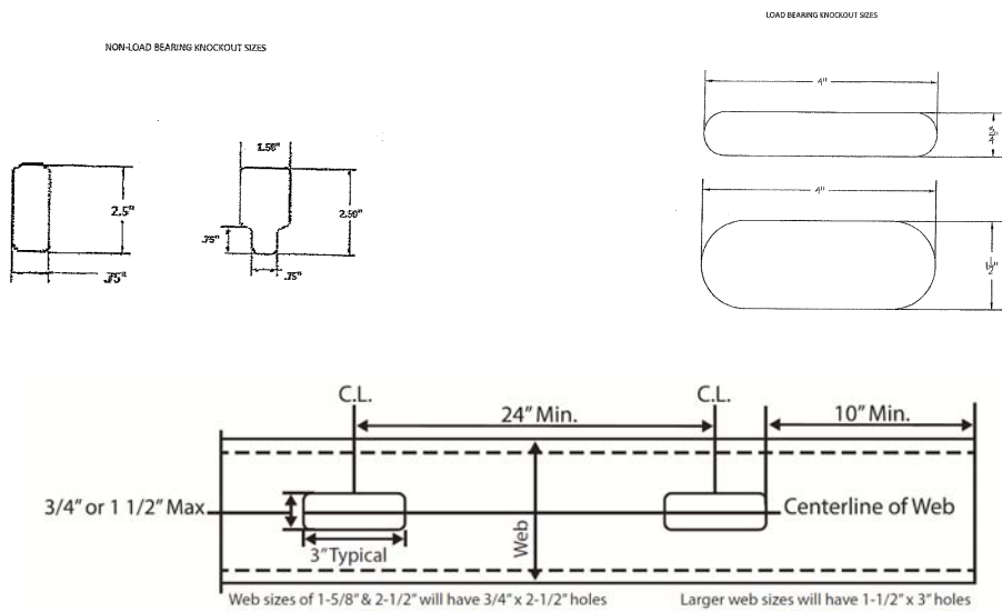
FIGURE 2—PUNCH-OUTS
