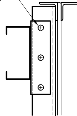
SECTION VIEW
