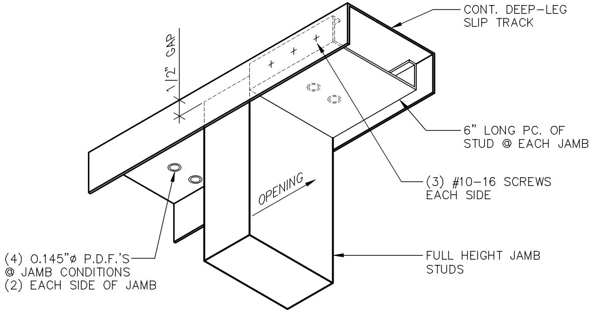
@ JAMB CONDITIONS
