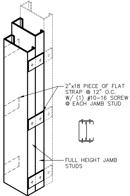
SCREWED OPTION
