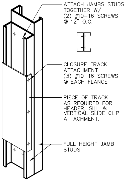
SCREWED OPTION
