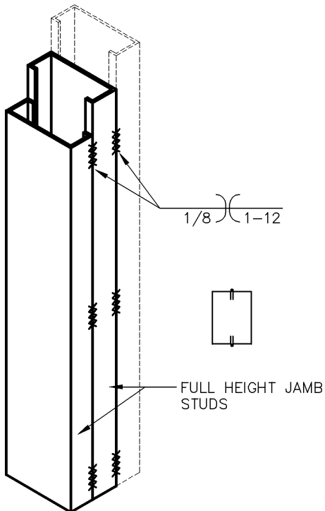
WELDED OPTION
